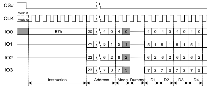
Figure 7.21 Word Read Quad I/O Instruction(Initial command or previous M5-4 ≠10)
