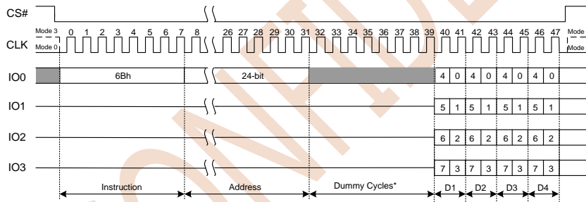
Figure 7.16 Fast Read Quad Output Instruction
