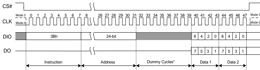
Figure 7.15 Fast Read Dual Output Instruction Sequence Diagram
