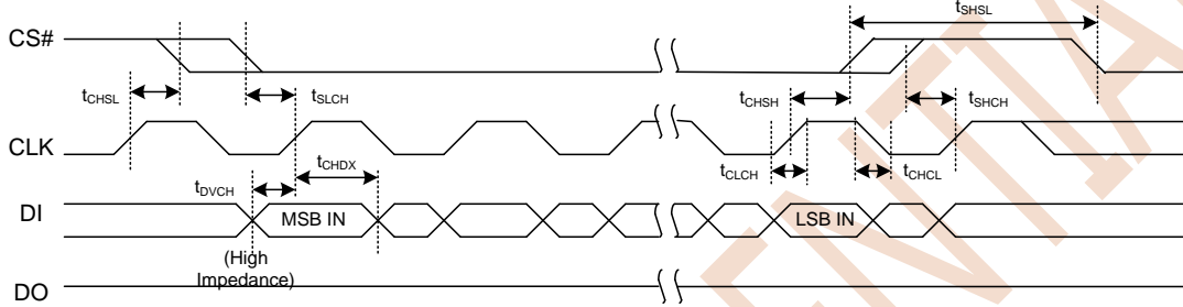
Figure 8.5 Input Timing
