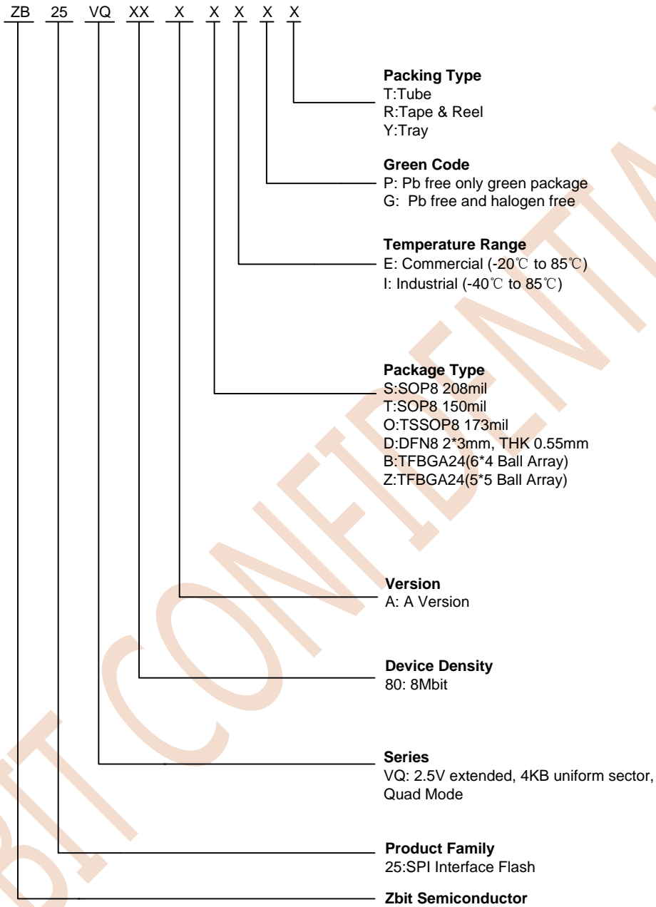
Figure 1.1 Ordering Information
