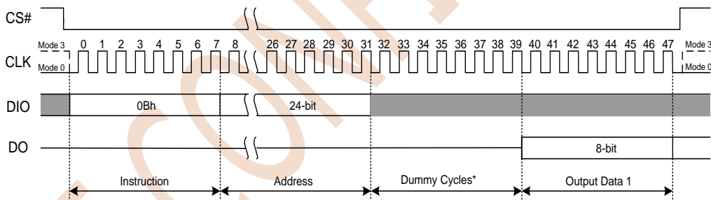
Figure 7.14a Fast Read Instruction
