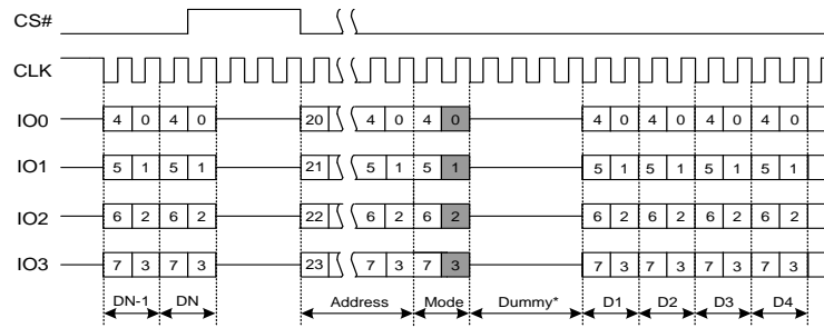
Figure 7.20 Fast Read Quad I/O Instruction(Previous command set M5-4 = 10)
