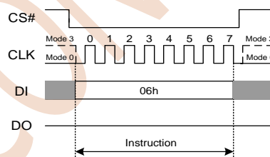
Figure 7.2 Write Enable Instruction
